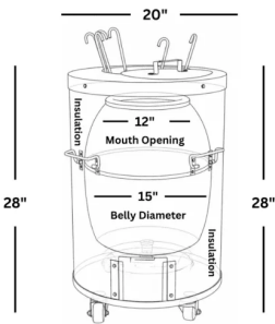
Wireframe — Dimensions & Insulation Cross-Section
