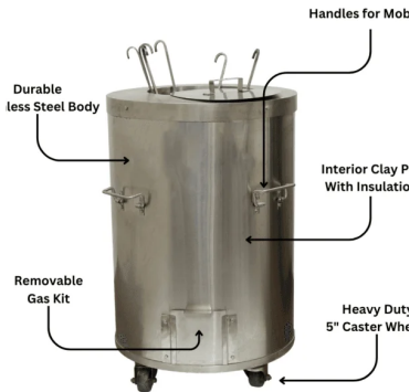
Features — Labeled Component View
