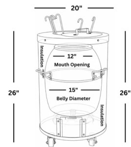
Wireframe — Dimensions & Insulation Cross-Section
